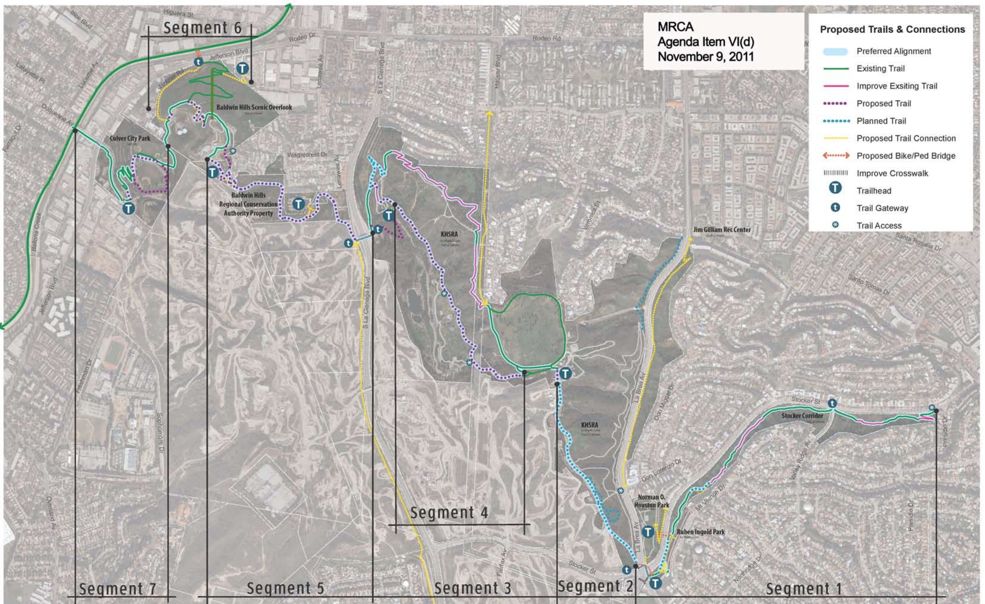
Park to Playa Trail Proposed Alignment
